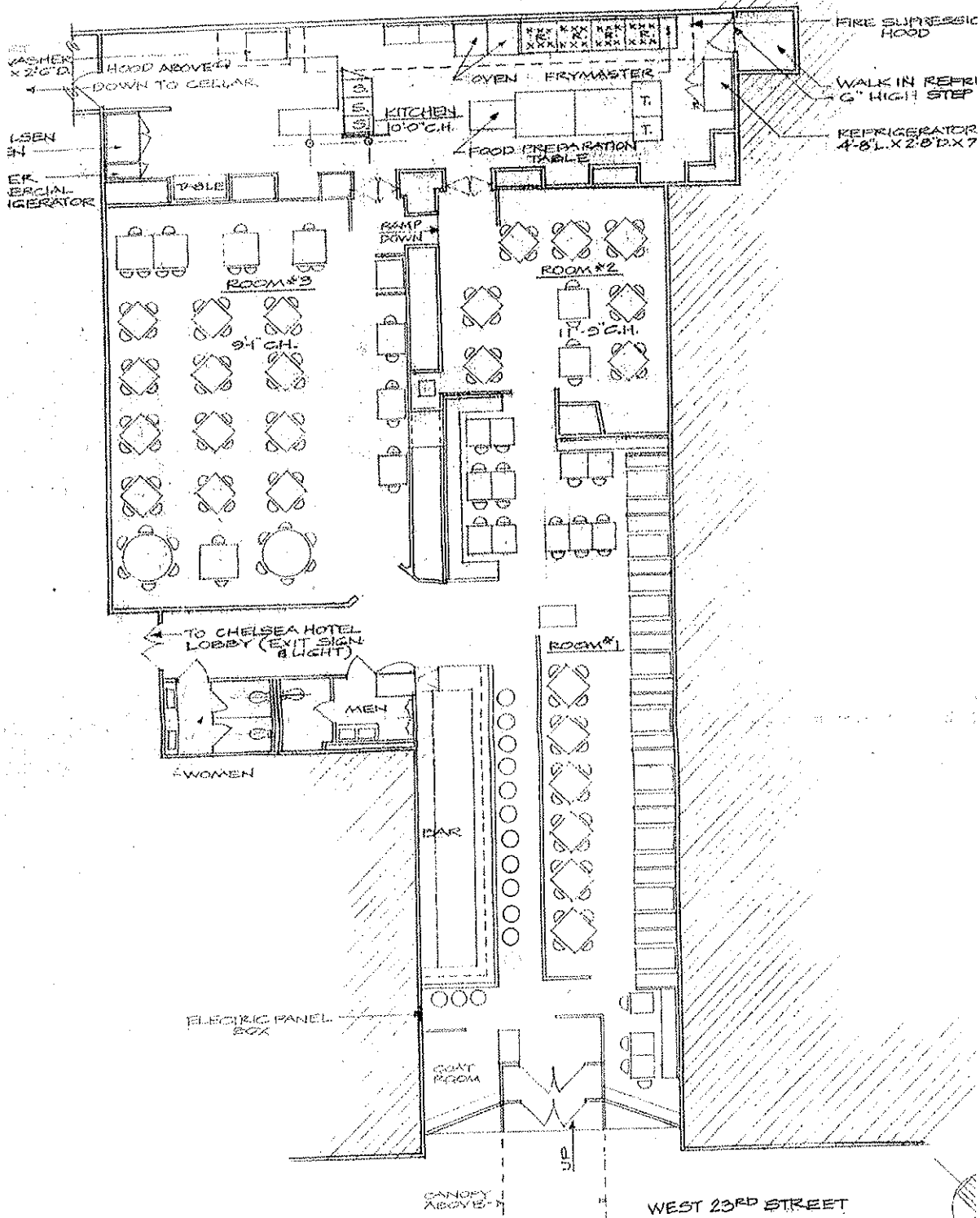
GROUND FLOOR PLAN OF EL QUIJOTE RESTAUR. 226 WEST 23RD STREET NEW YORK, N.Y. 10011 SCALE: \frac{1}{8}'' = 1'-0''
