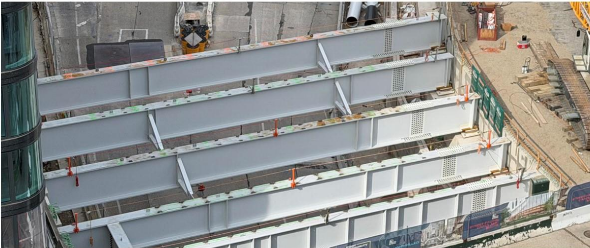
Steel Girder Installation over the LTE (6/19/26)
