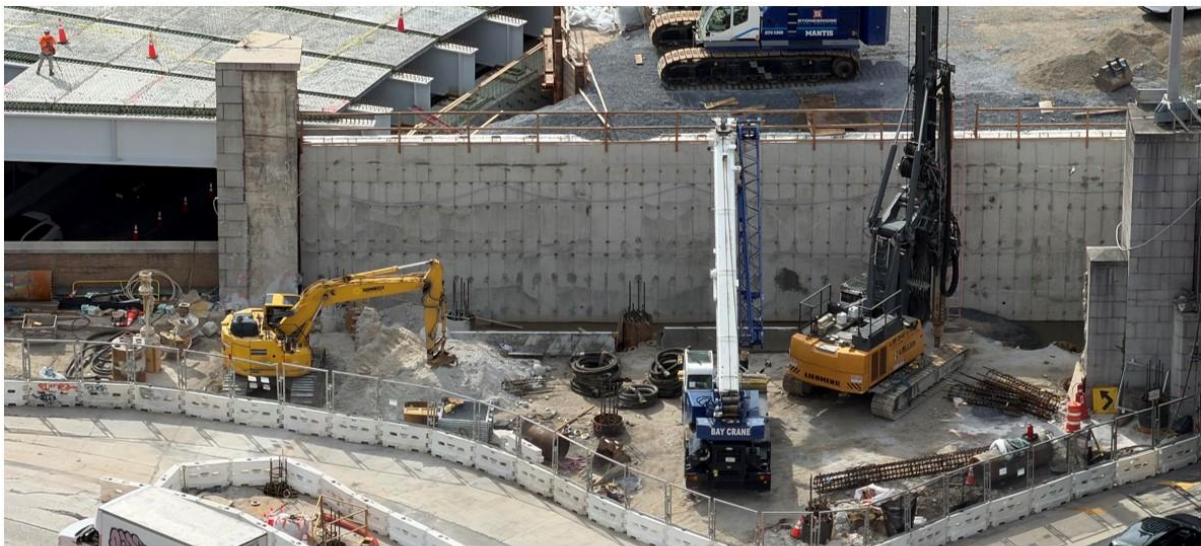
Drilled Shafts in Dyer Plaza (6/19/26)
