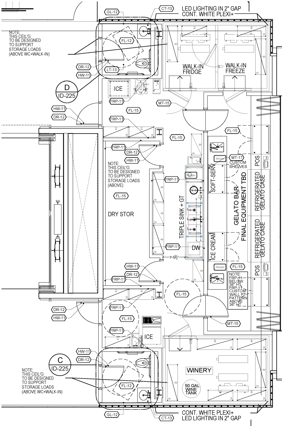
FLOOR PLAN at CONCESSION STAND
