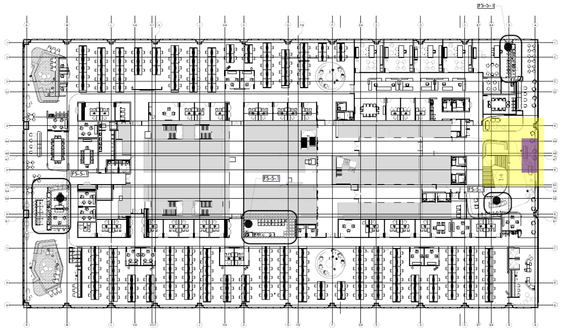
1 5th FLOOR - OVERALL FOODSERVICE EQUIPMENT PLAN SCALE: 3/32" = 1'-0"
