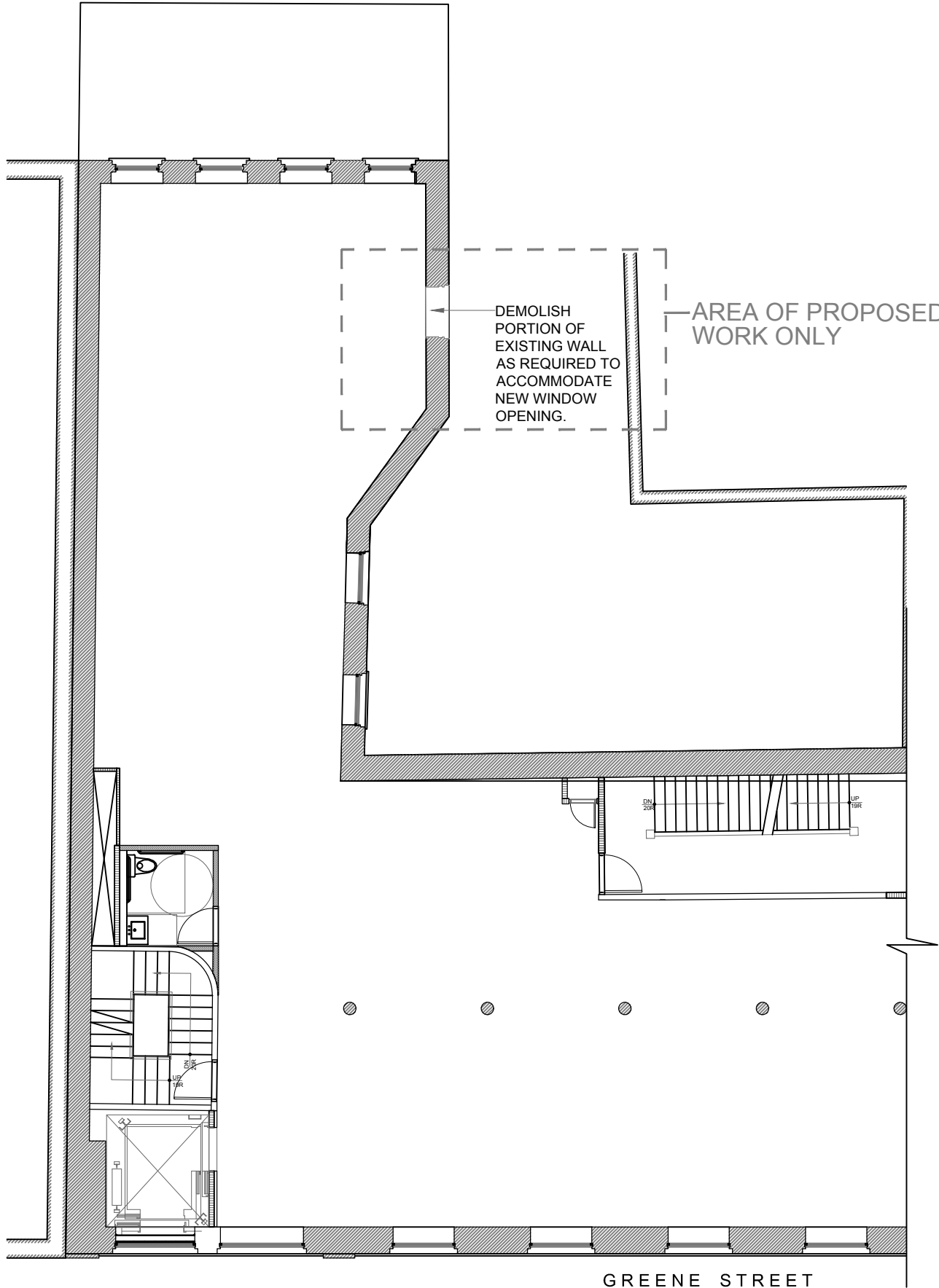
1 EXISTING SECOND - SIXTH FLOOR PARTIAL PLAN SCALE 3/32"=1'-0"
