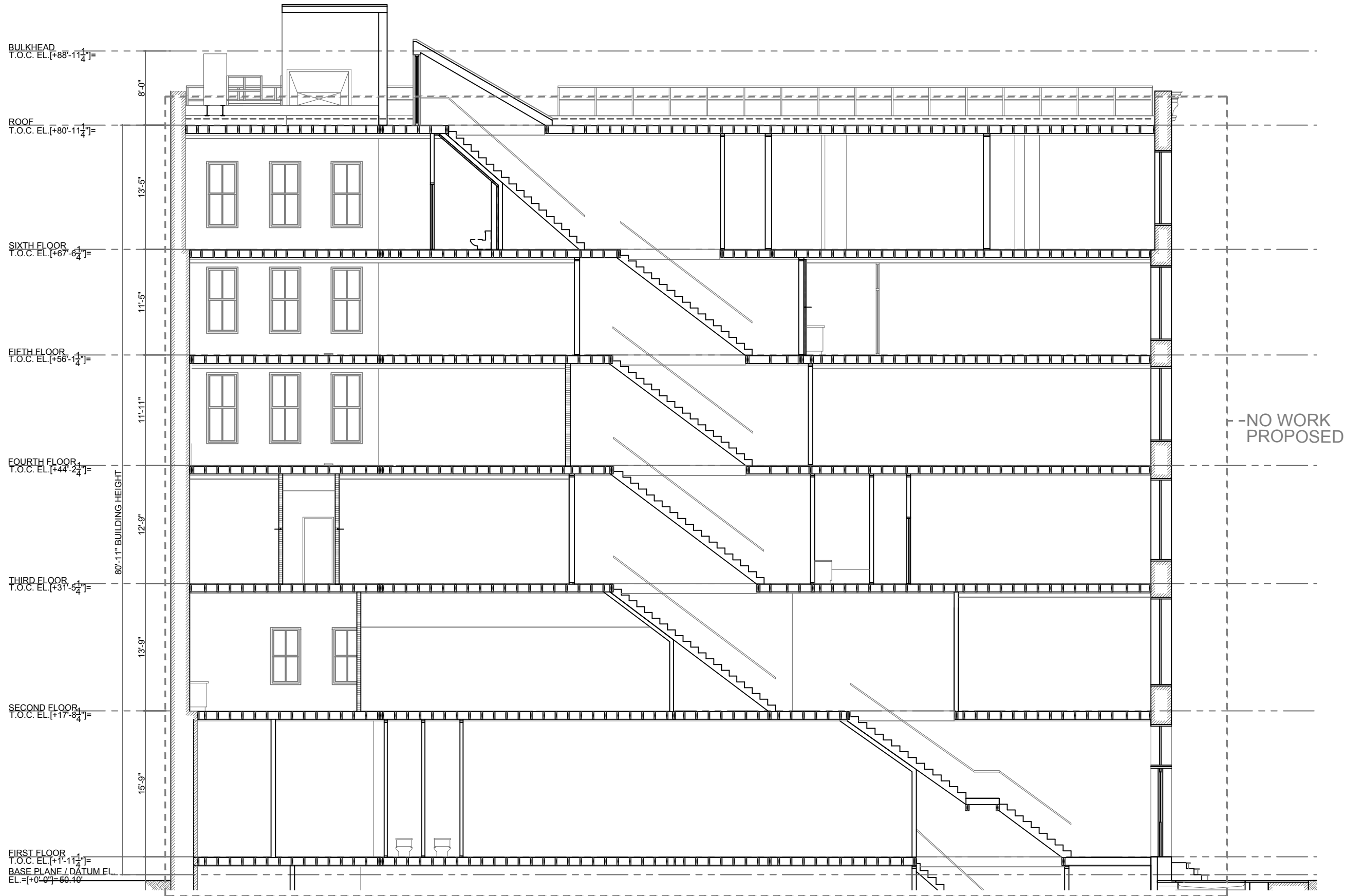
1 EXISTING SECTION SCALE 3/32"=1'-0"
