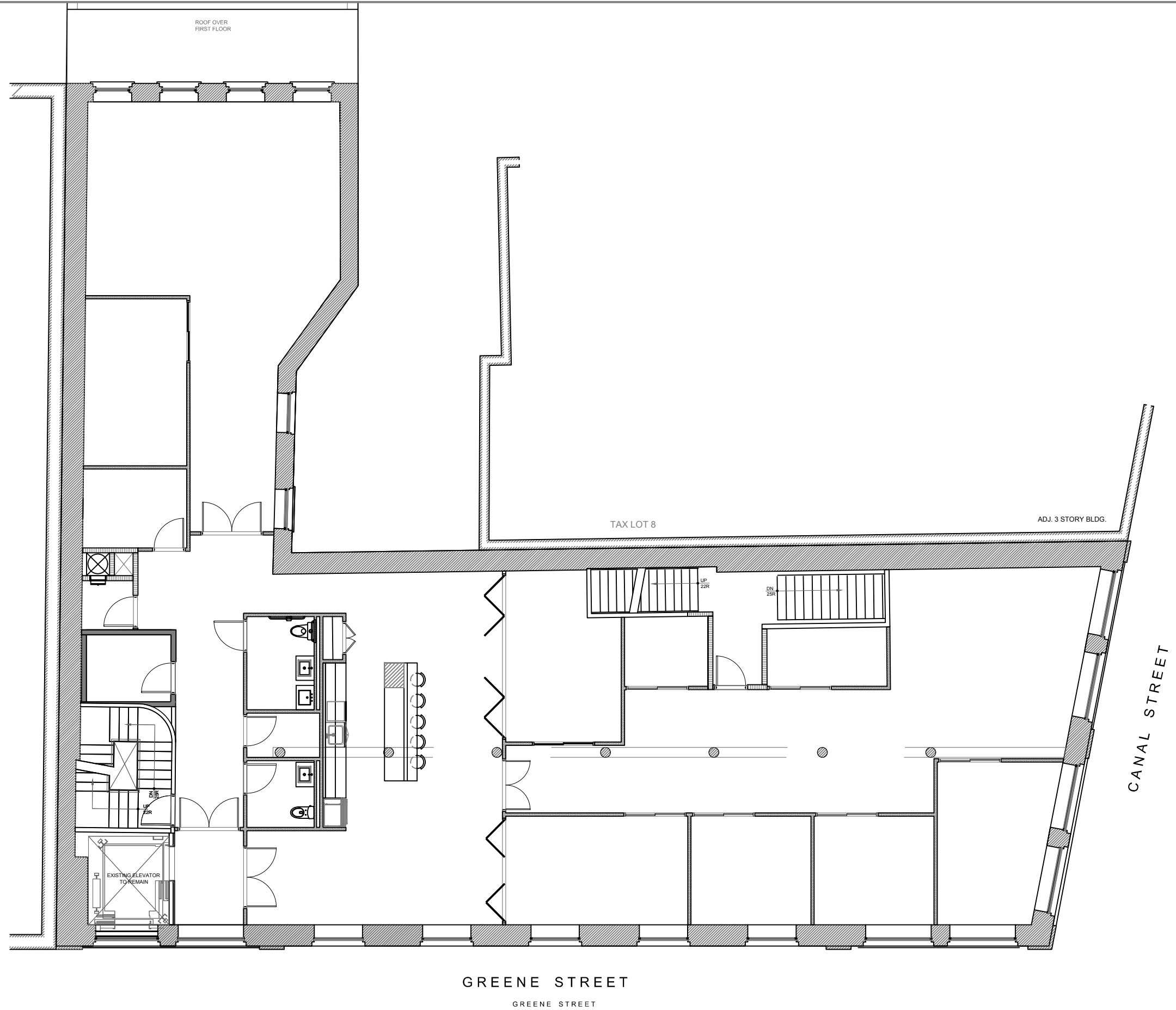
1 PROPOSED SECOND FLOOR PLAN SCALE 3/32"=1'-0"
