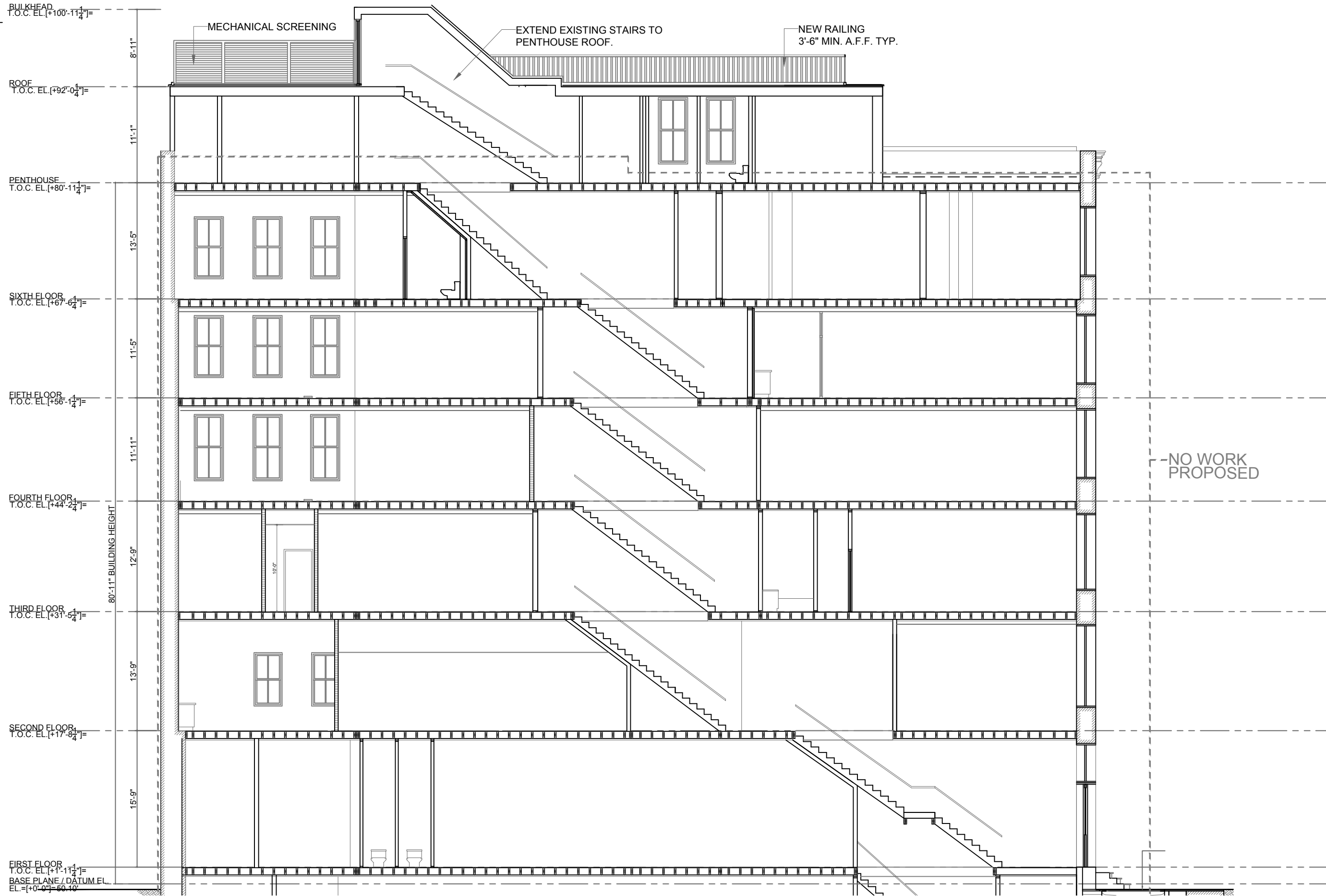
1 PROPOSED SECTION SCALE 3/32"=1'-0"
