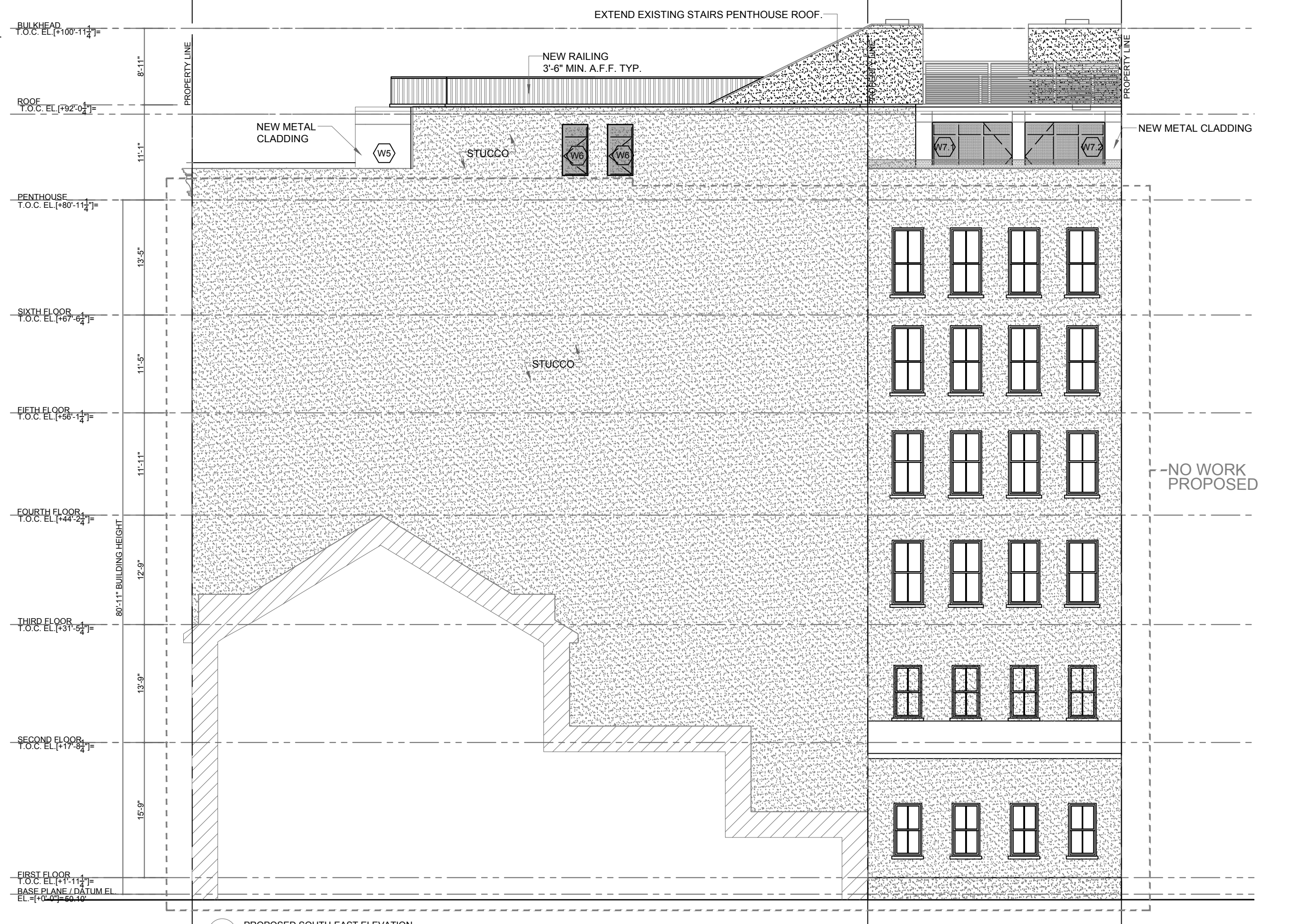
1 PROPOSED SOUTH-EAST ELEVATION SCALE 3/32"=1'-0"
