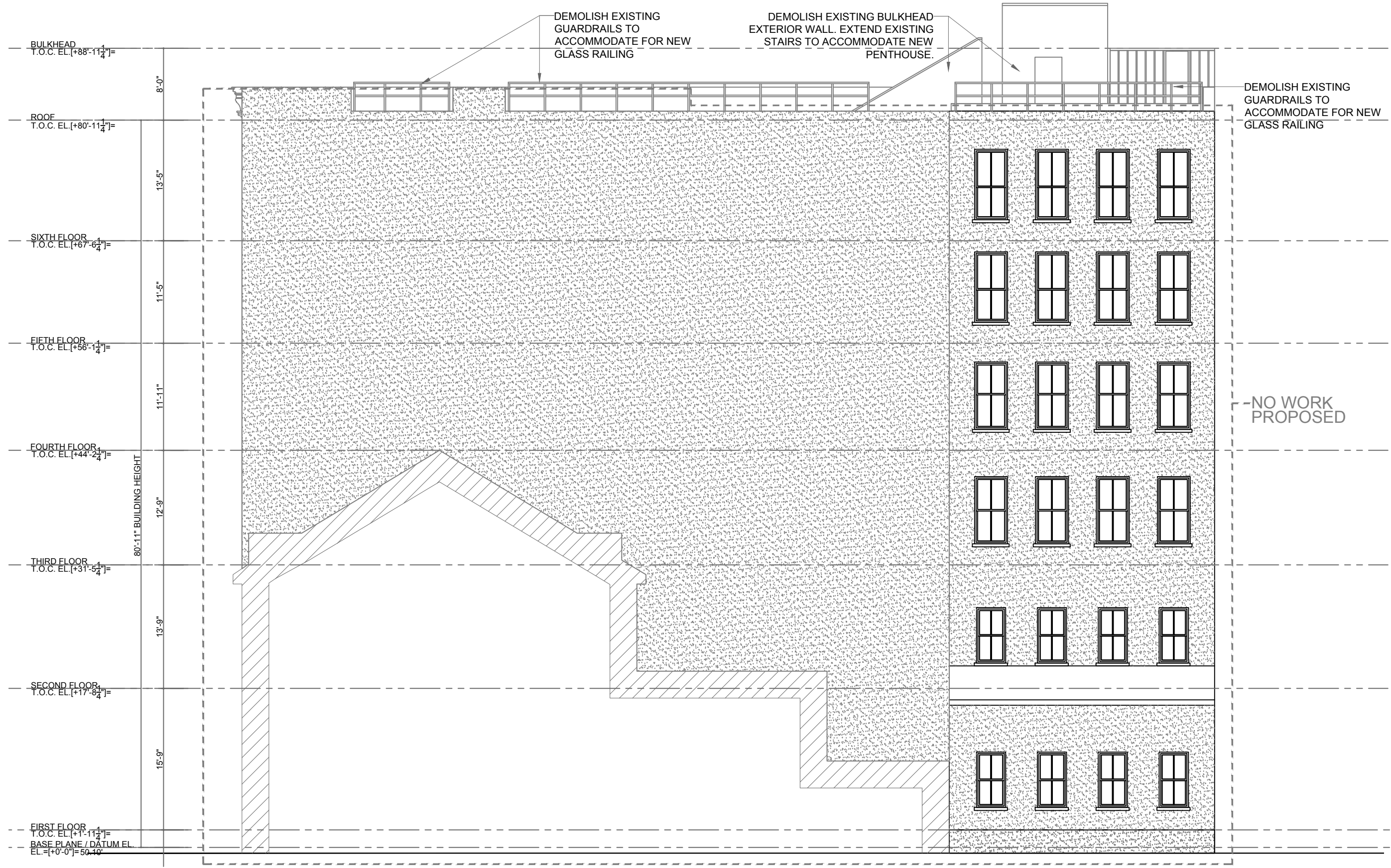
1 EXISTING SOUTH-EAST ELEVATION SCALE 3/32"=1'-0"
