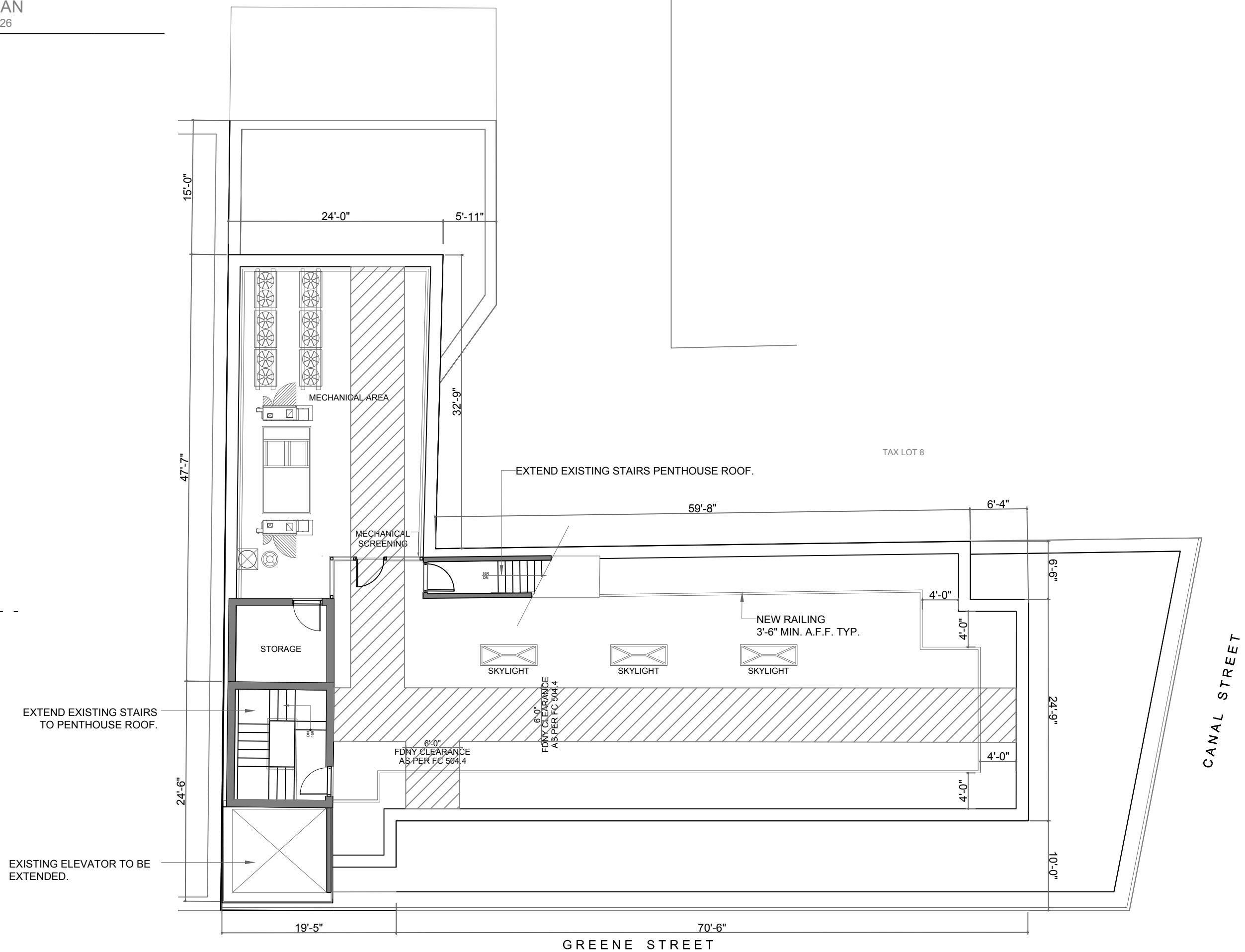
1 PROPOSED ROOF PLAN SCALE 3/32"=1'-0"
