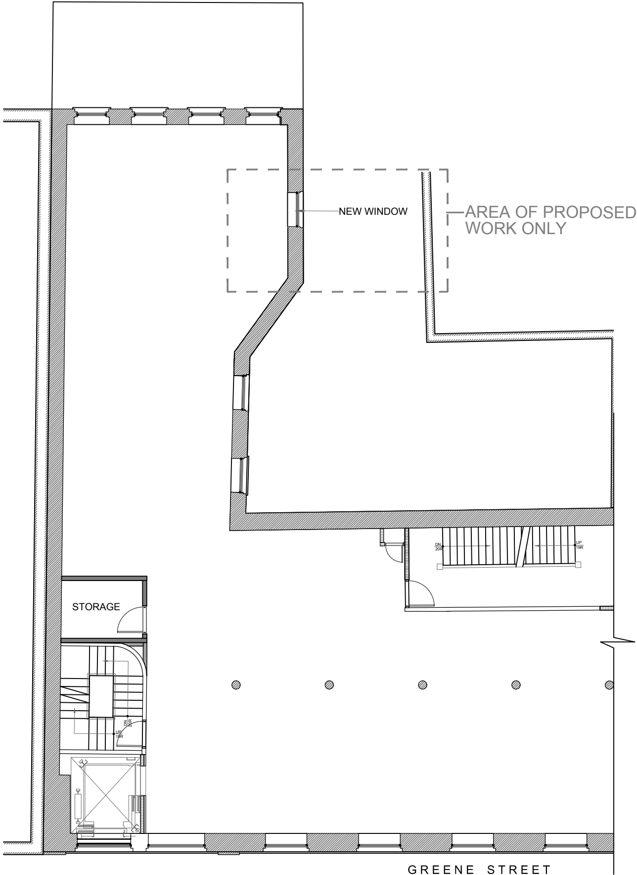
2 PROPOSED SECOND - SIXTH FLOOR PARTIAL PLAN SCALE 3/32"=1'-0"
