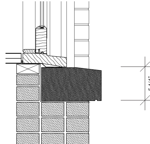
Proposed Sill Detail
