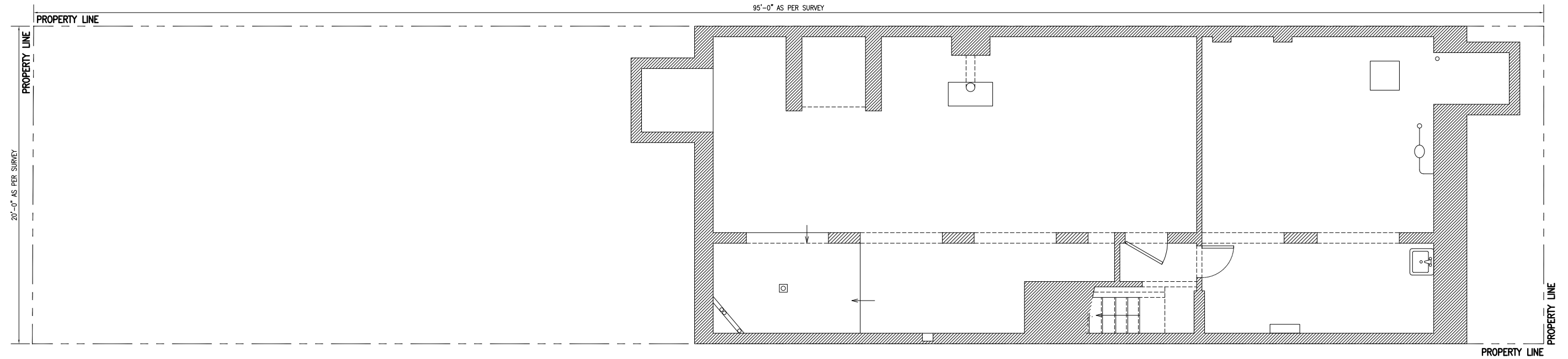
Existing Cellar Plan
