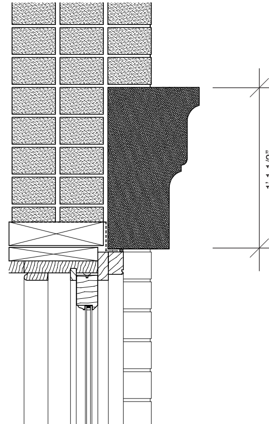
Proposed Lintel Detail
