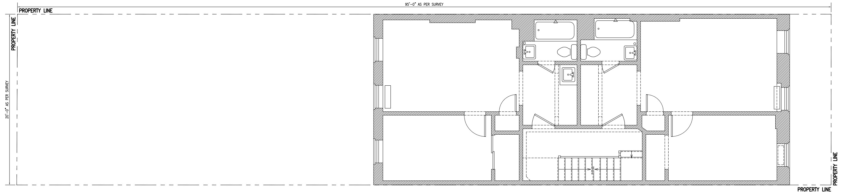
Existing First Floor Plan
