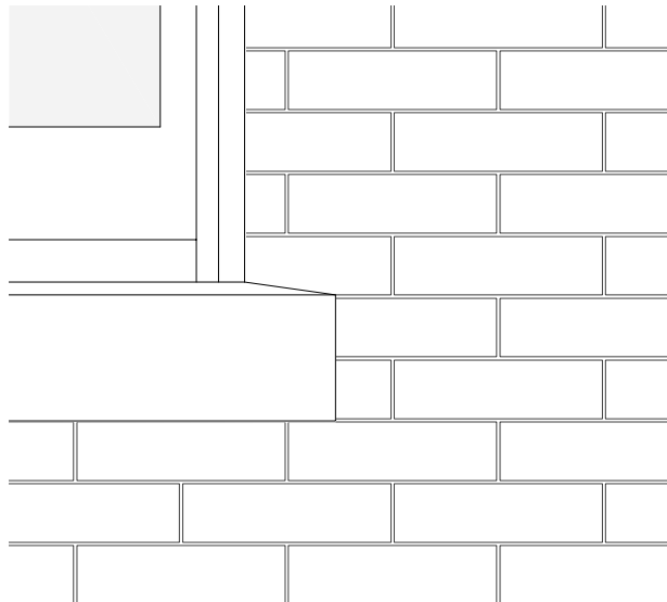
Proposed Sill Detail
