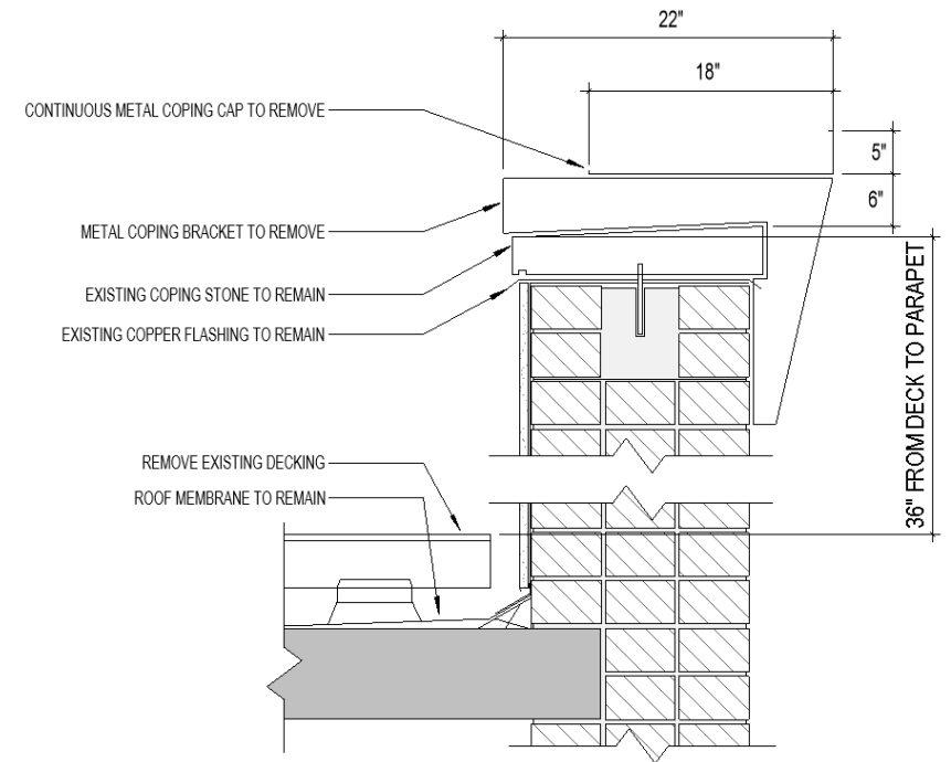
PARAPET SECTION
