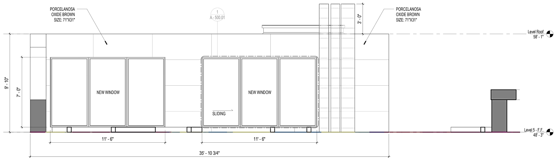
PROPOSED ELEVATION
