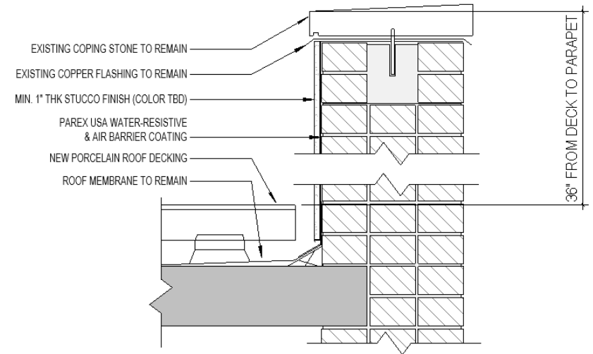
PARAPET SECTION
