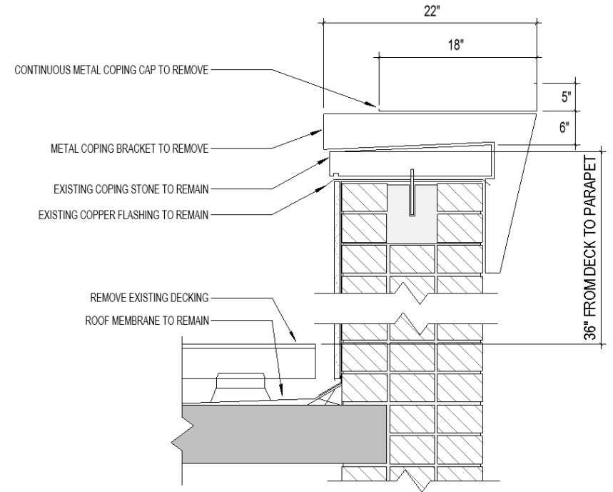
PARAPET SECTION
