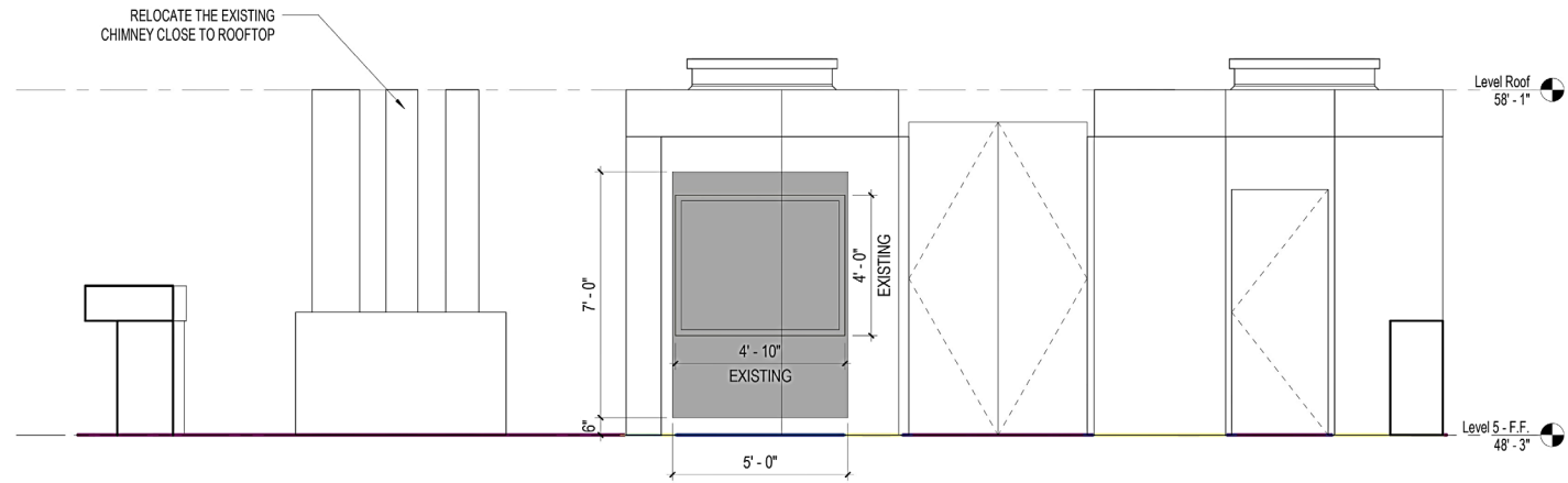
EXISTING ELEVATION
