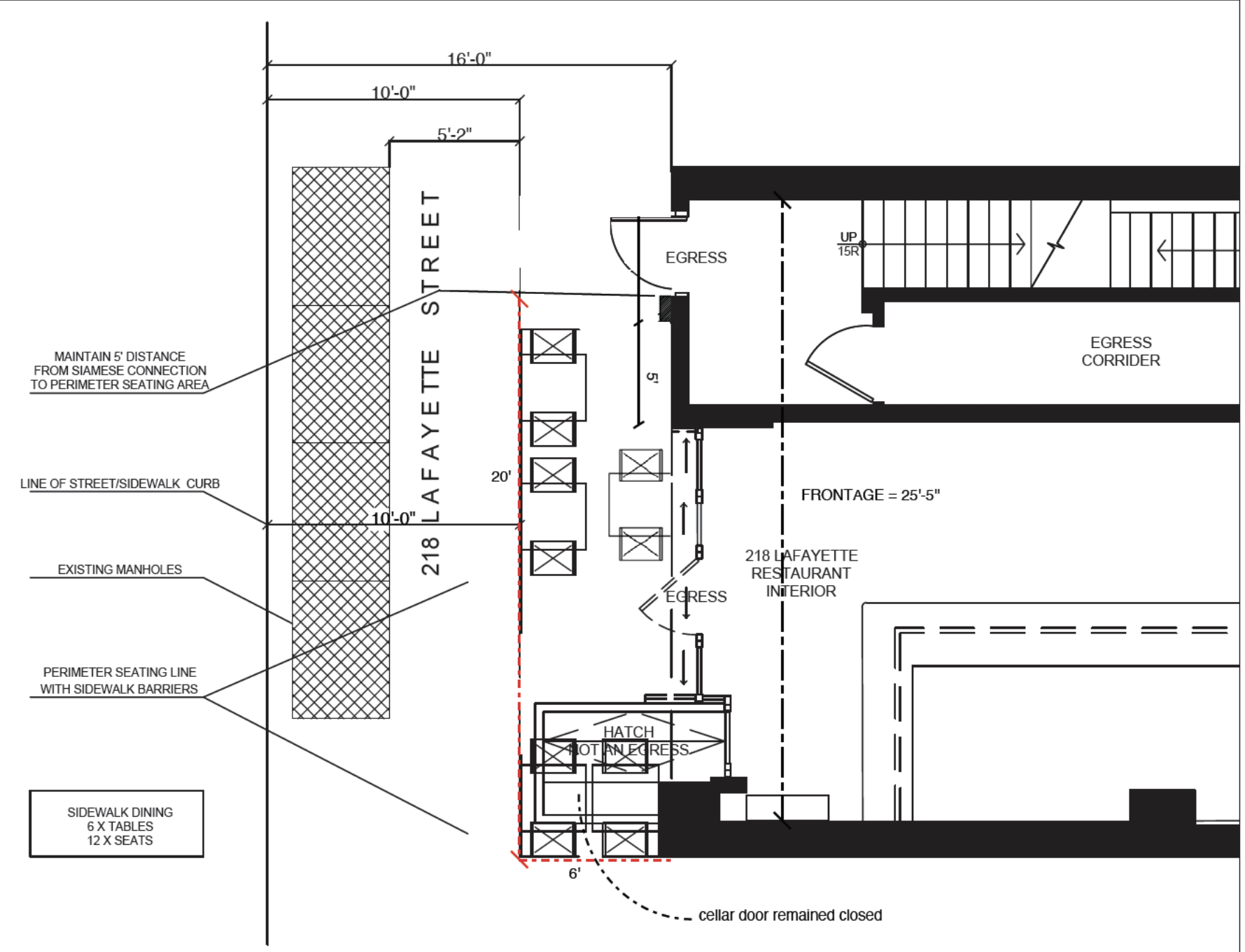
CRAZY PIZZA - 218 LAFAYETTE SIDEWALK CAFE PLAN 2025
