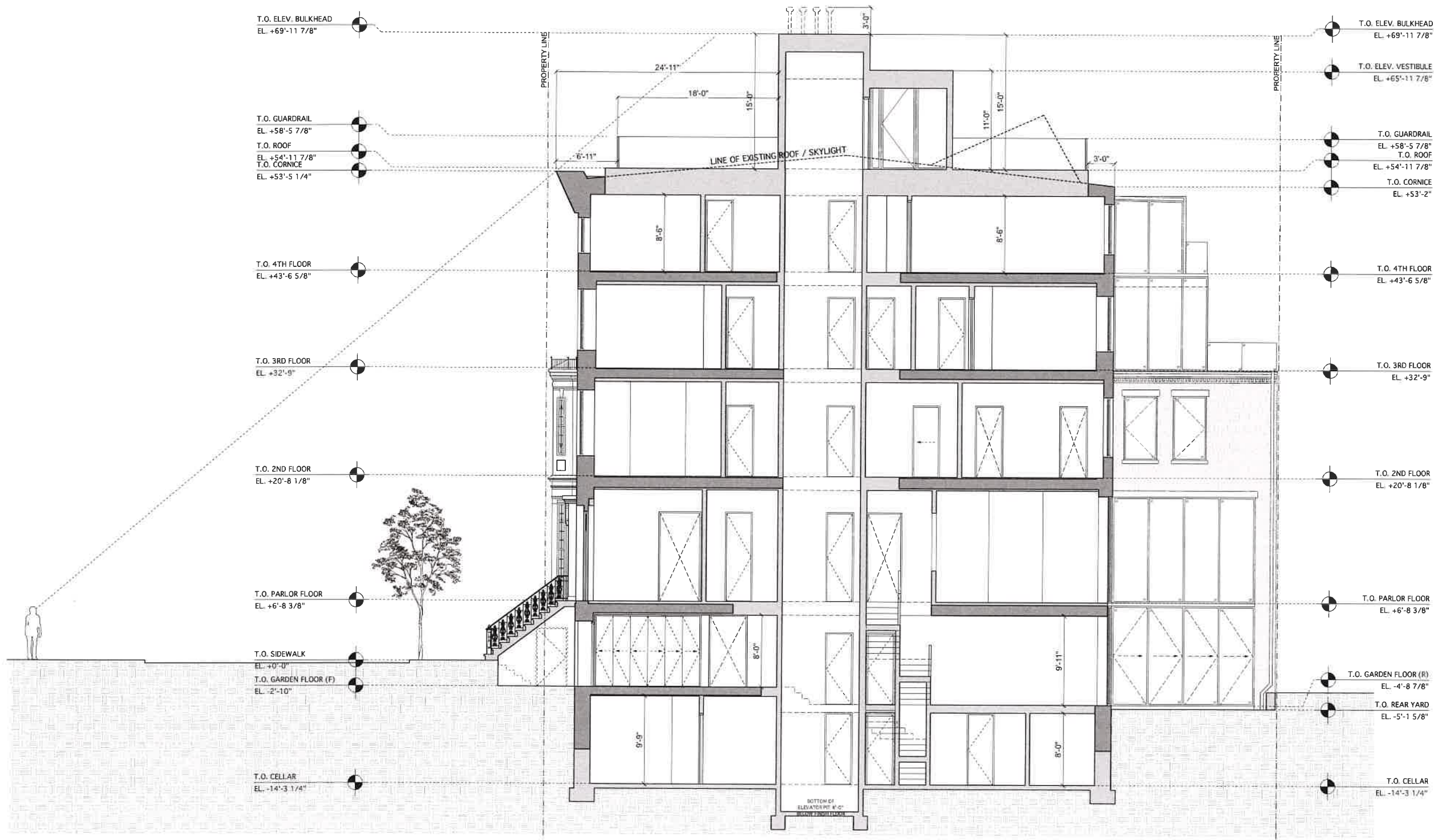
1 PROPOSED BUILDING SECTION
