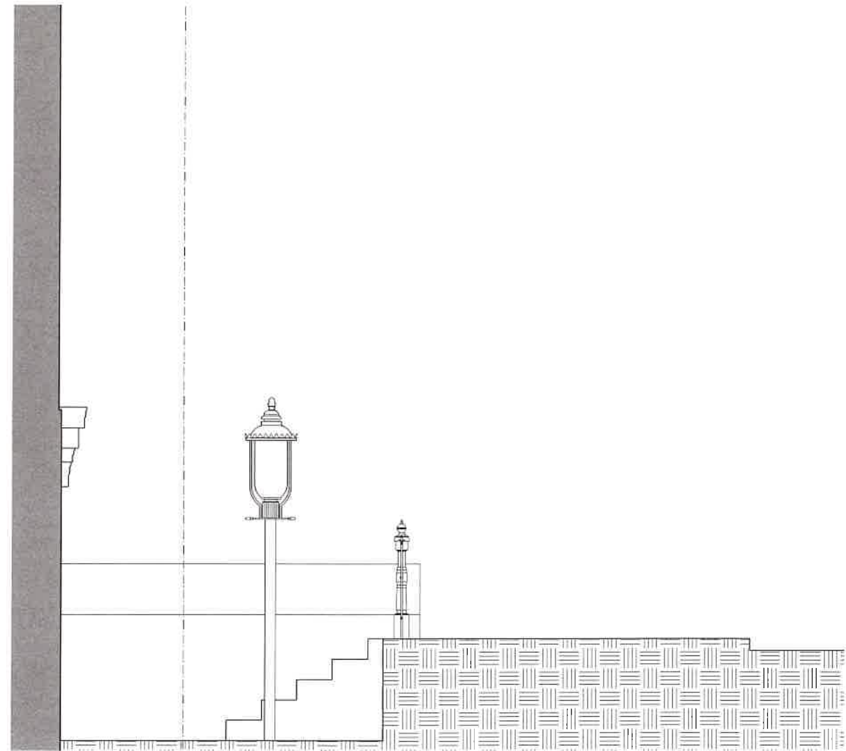
2 EXISTING AREAWAY WEST ELEVATION
