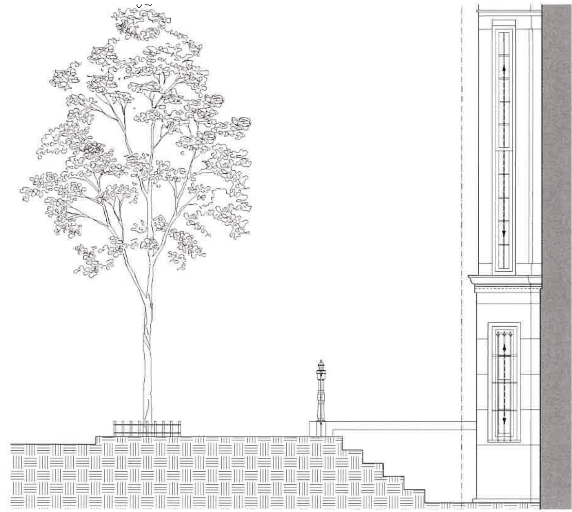
1 PROPOSED AREAWAY & STOOP EAST ELEVATION
