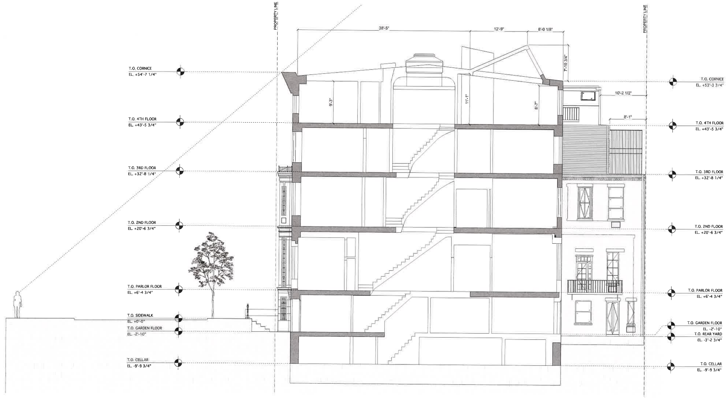
EXISTING BUILDING SECTION
