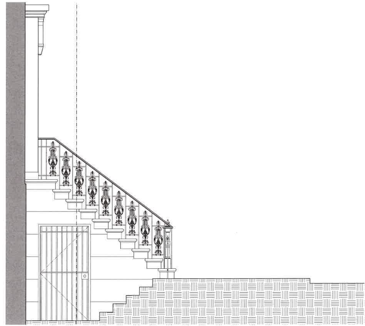
1 PROPOSED AREAWAY & STOOP WEST ELEVATION
