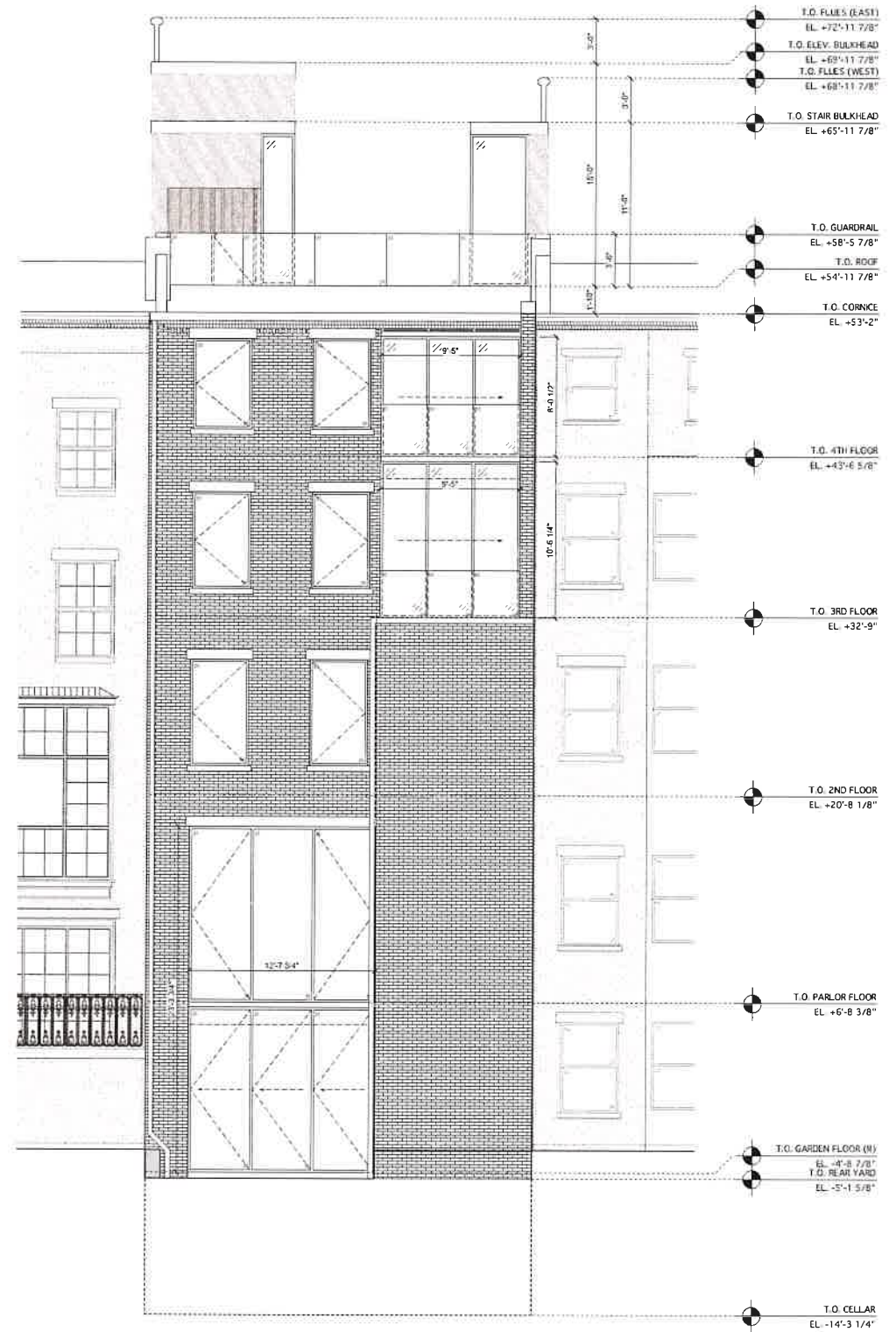
1 PROPOSED REAR ELEVATION
