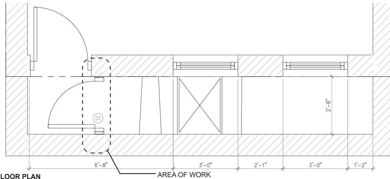
PROPOSED CELLAR FLOOR PLAN
