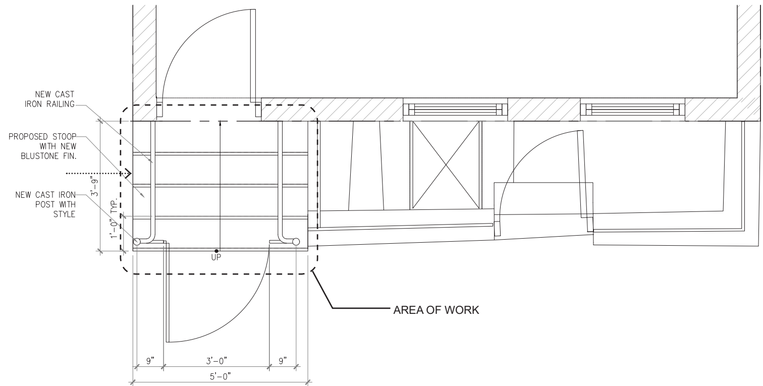
PROPOSED ENTRANCE FLOOR PLAN
