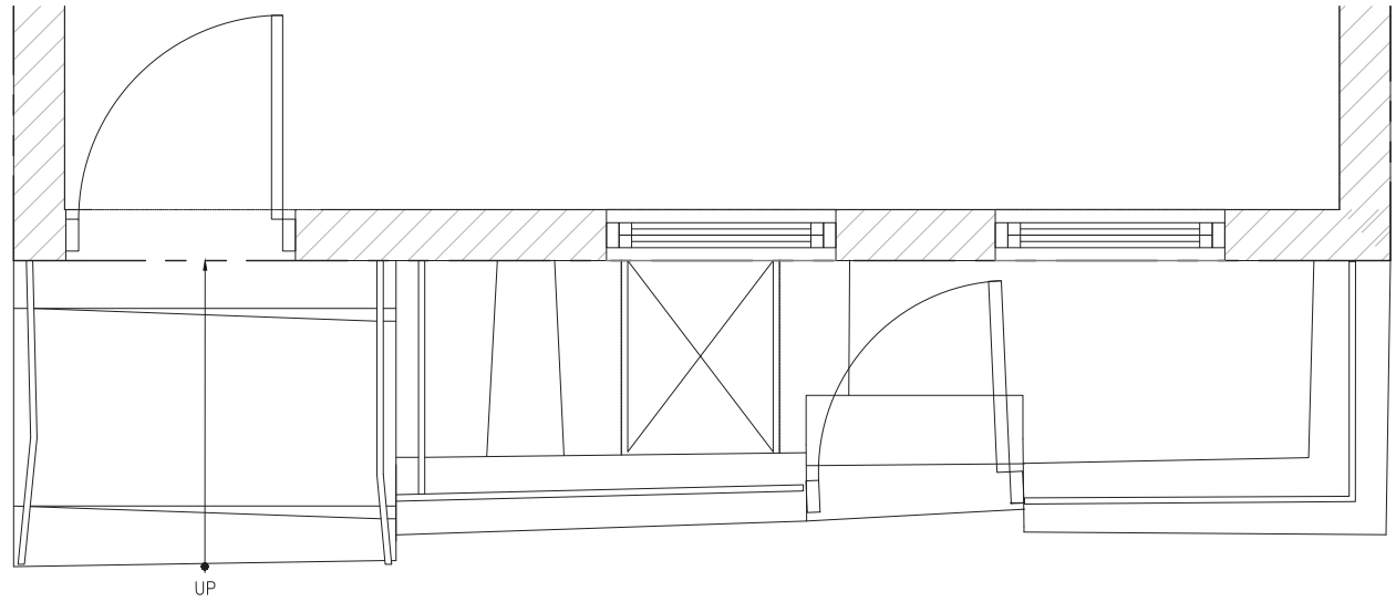
EXISTING ENTRANCE FLOOR PLAN
