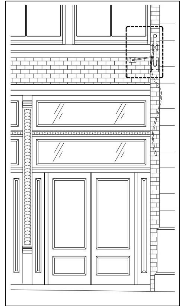
134 Spring Street, proposed partial elevation.
