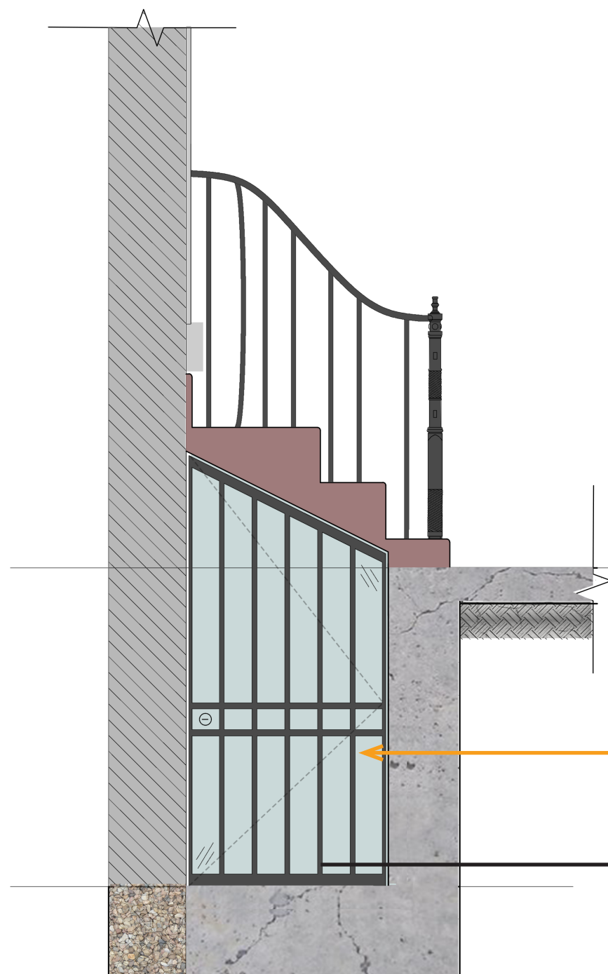
CELLAR ENTRANCE SECTION
