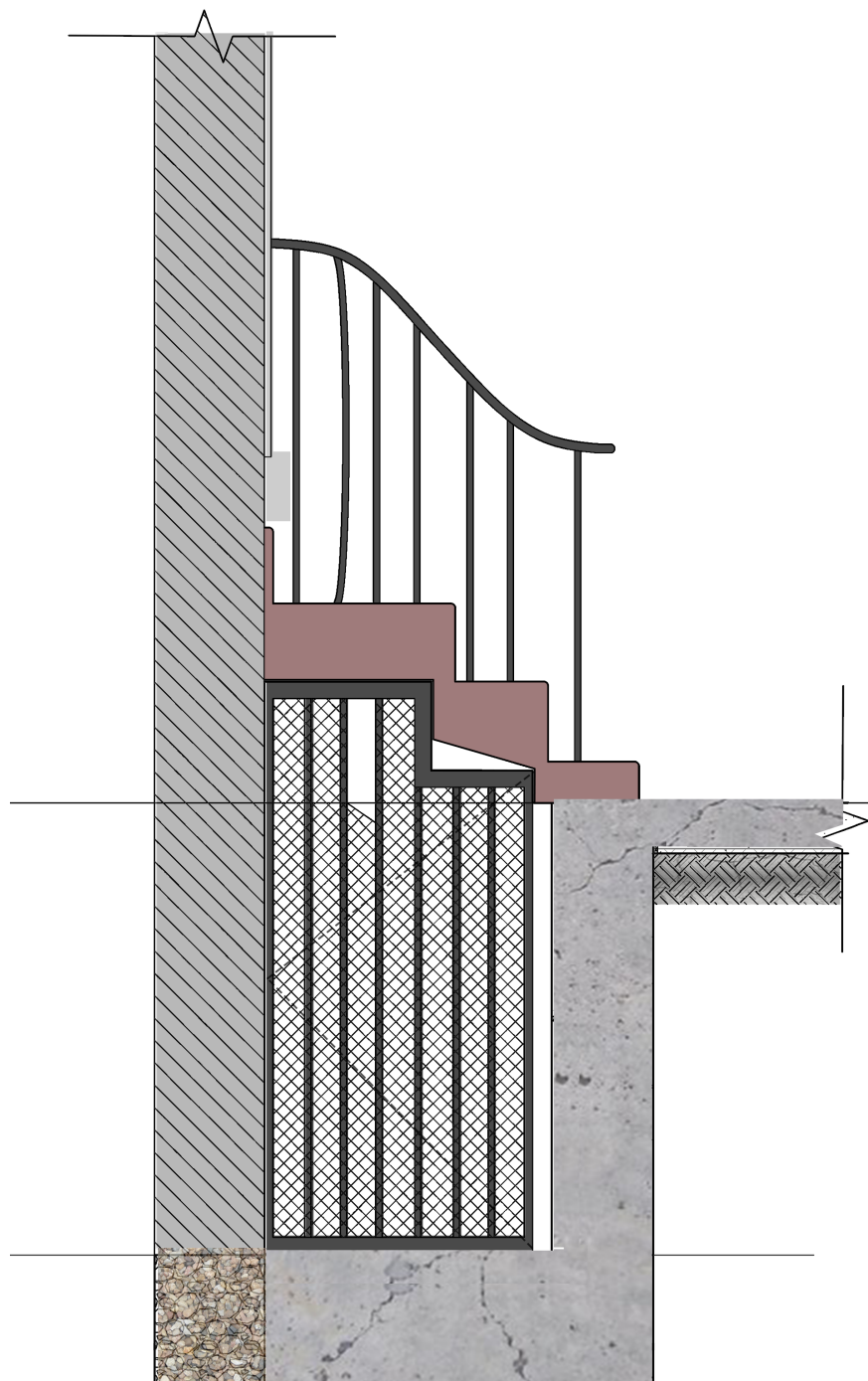
EXISTING CELLAR ENTRANCE SECTION
