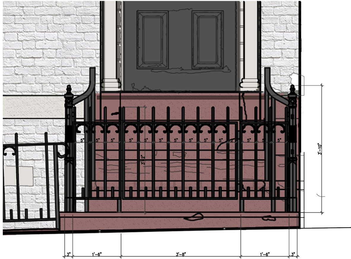
PROPOSED ENTRANCE ELEVATION WITH OPEN GATE
