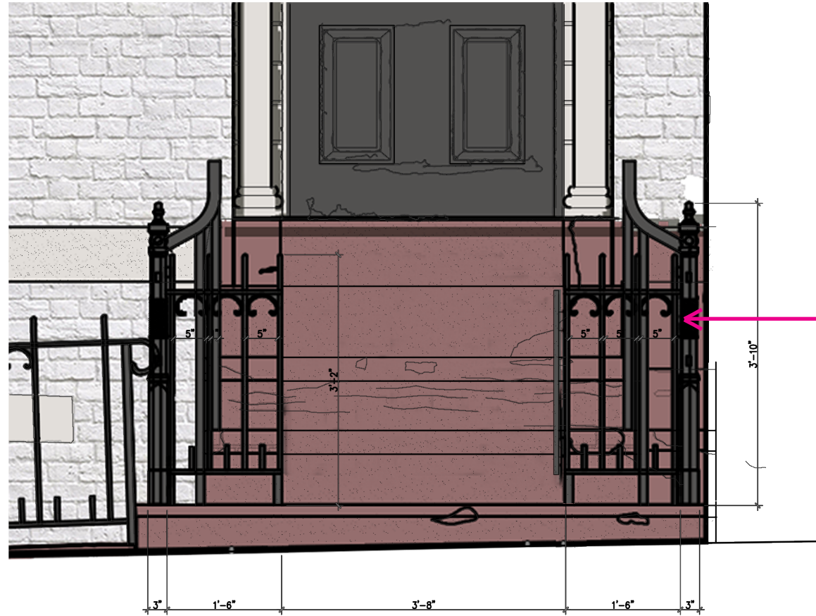
PROPOSED ENTRANCE ELVATION WITH CLOSED GATE
