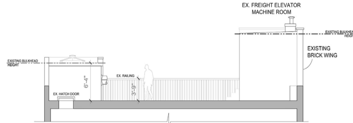
3 EXISTING WESTERN SECTIONAL ELEVATION SCALE: 1/8"=1'-0"
