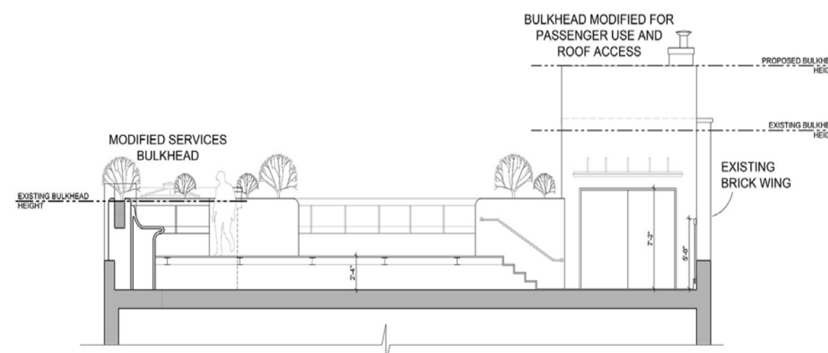
4 PROPOSED WESTERN SECTIONAL ELEVATION SCALE: 1/8"=1'-0"
