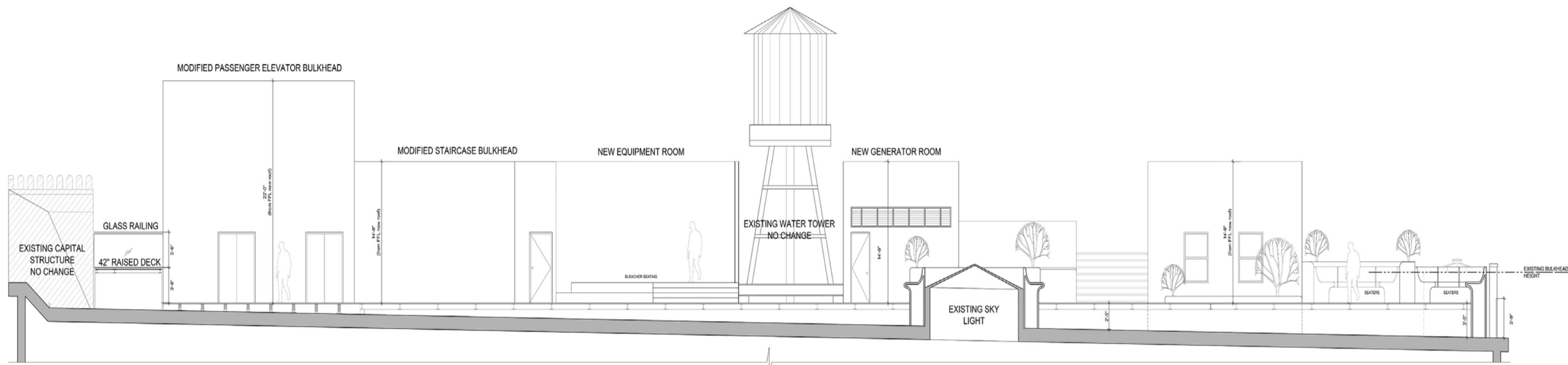
2 PROPOSED SOUTHERN SECTIONAL ELEVATION SCALE: 1/8"=1'-0"
