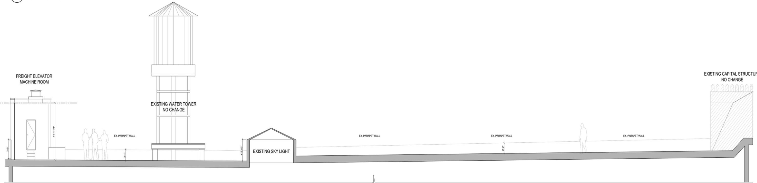
3 EXISTING NORTHERN SECTIONAL ELEVATION SCALE: 1/8"=1'-0"
