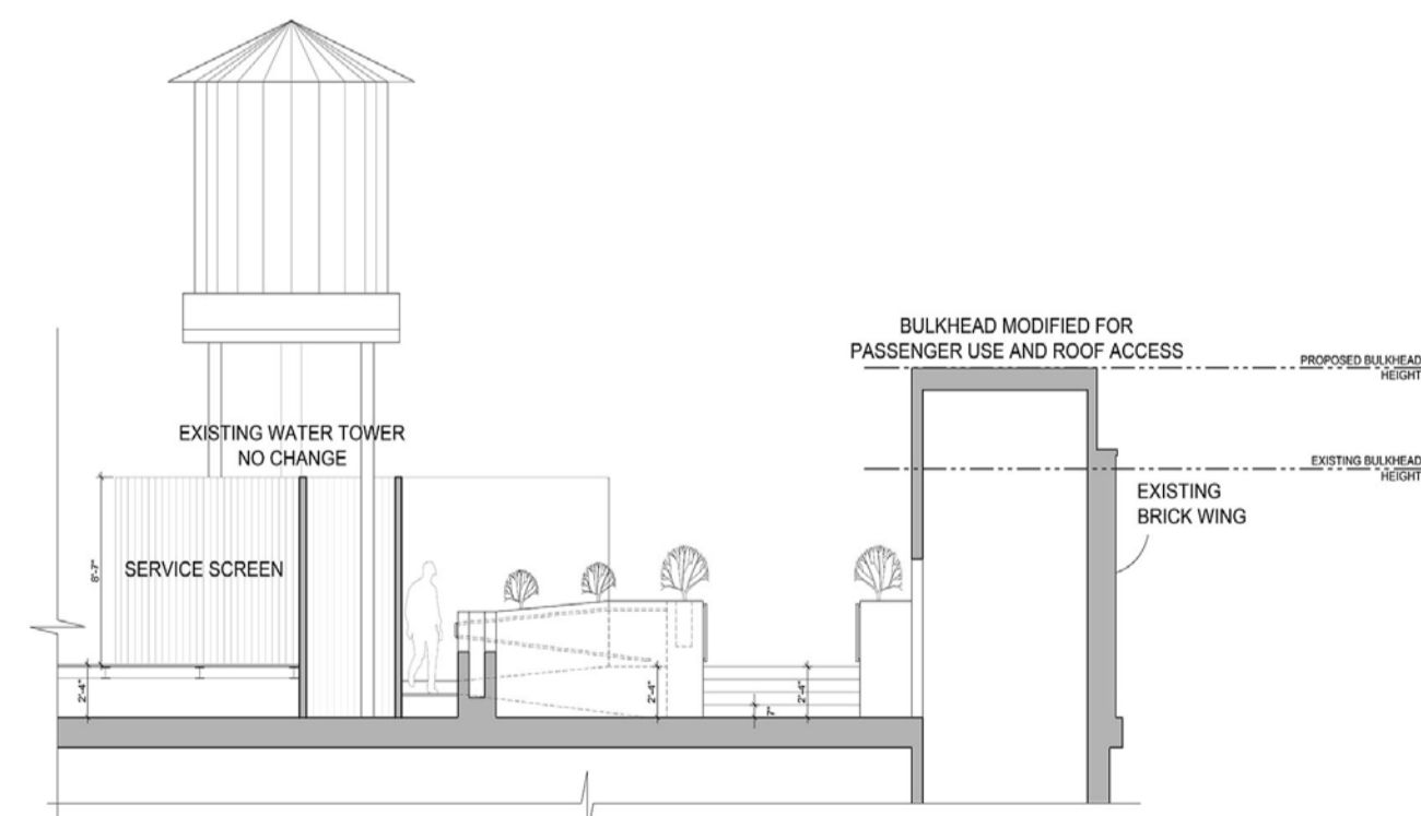
6 PROPOSED PART SOUTHERN SECTIONAL ELEVATION SCALE: 1/8"=1'-0"
