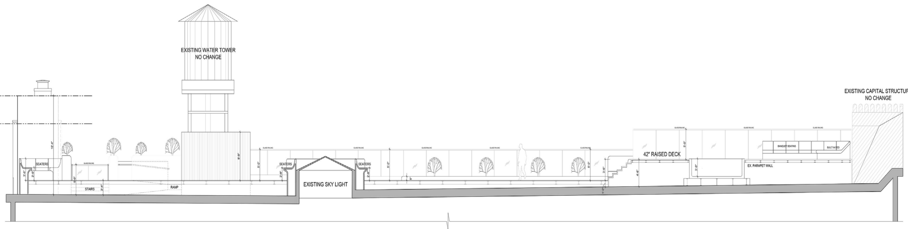
4 PROPOSED NORTHERN SECTIONAL ELEVATION SCALE: 1/8"=1'-0"
