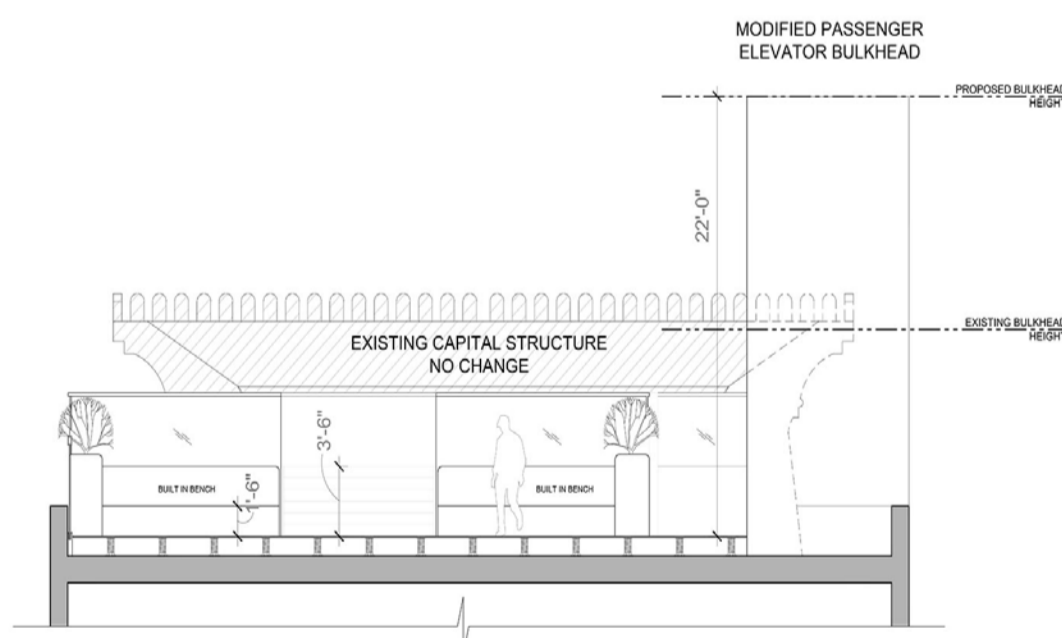
2 PROPOSED EASTERN SECTIONAL ELEVATION SCALE: 1/8"=1'-0"
