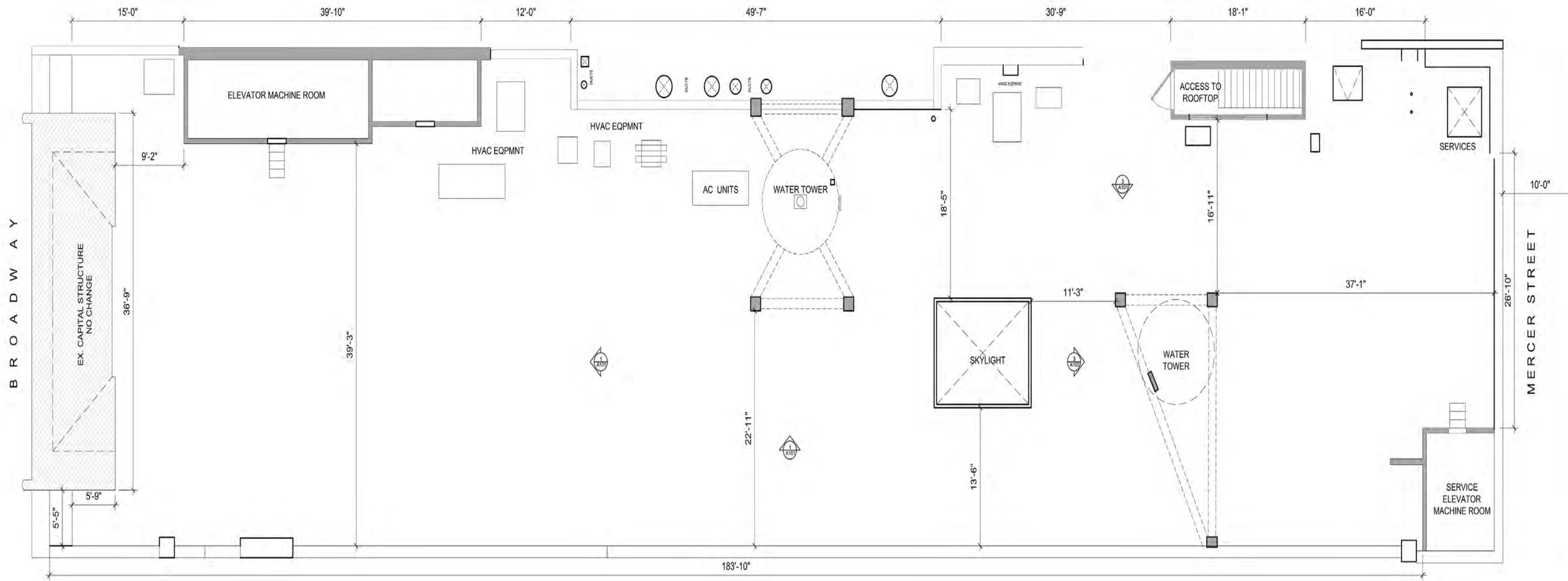
1 EXISTING ROOFTOP PLAN SCALE: 1/8"=1'-0"
