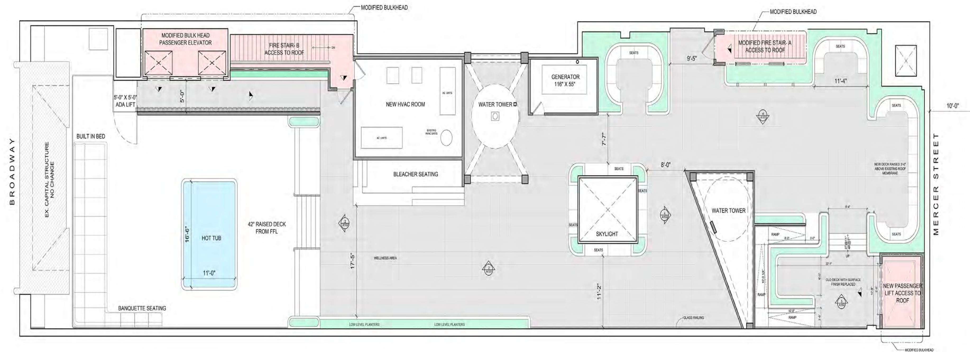
2 PROPOSED ROOFTOP PLAN SCALE: 1/8"=1'-0"
