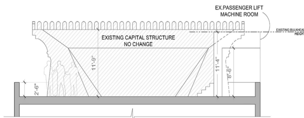
1 EXISTING EASTERN SECTIONAL ELEVATION SCALE: 1/8"=1'-0"
