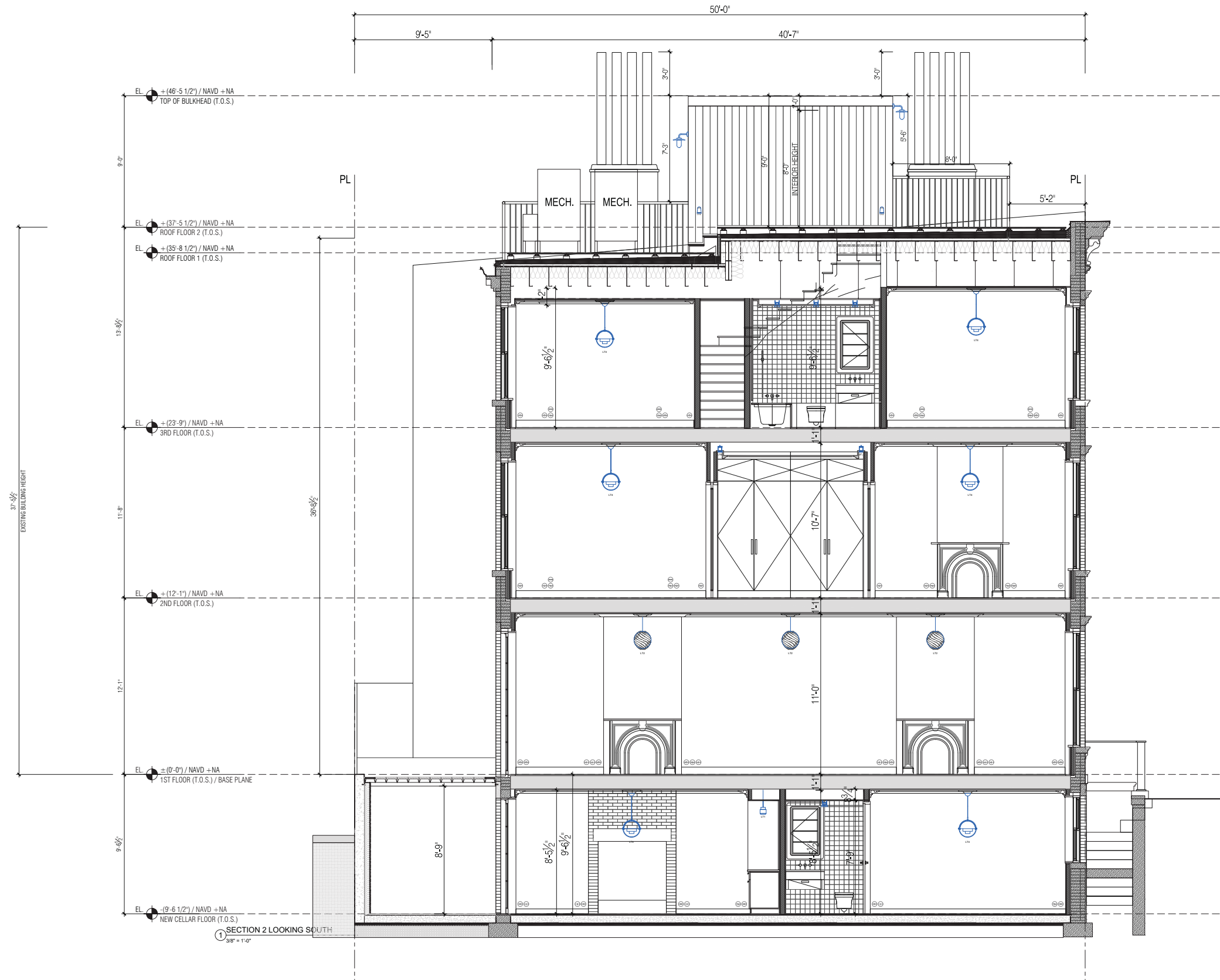
PROPOSED SECTION
