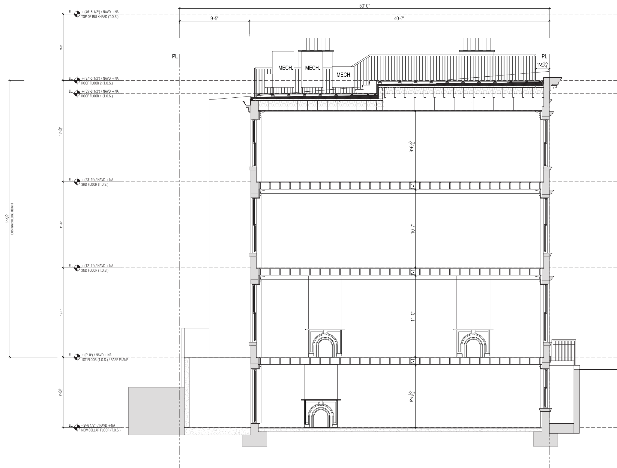
EXISTING SECTION
